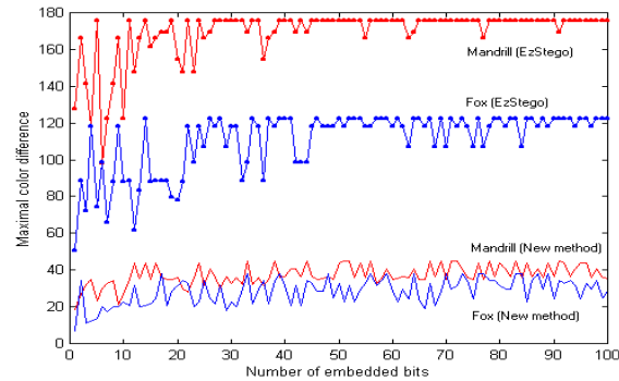
fig 9 Maximal color change caused by EZ Stego and the new technique.
