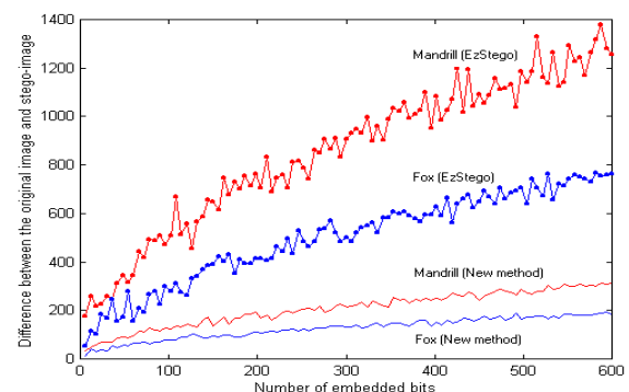
Fig 8 Comparison of distortion introduced by EZ Stego and the new technique.
